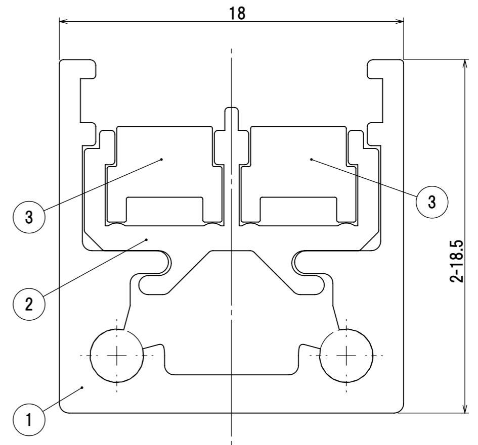
DETAIL A (5 : 1)
