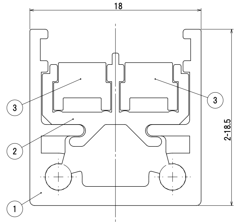
DETAIL A (5 : 1)
